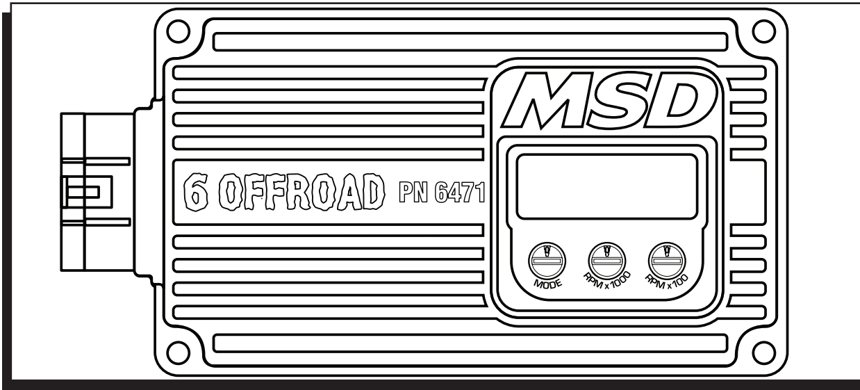
Figure 1 Off-Road Ignition Controller, PN 6471
