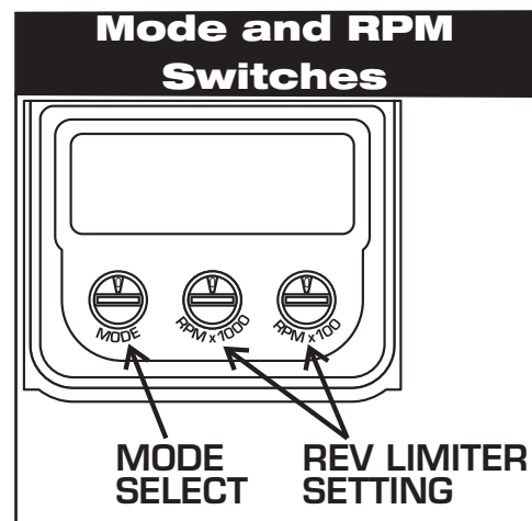
Figure 2 Mode and RPM Switches
